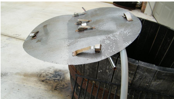
Left—The collapsed mash tun screen — couldn't stand up to 69.5 lbs of grain. <=====
